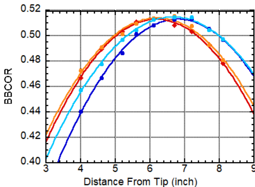
Figure 4 Comparison of BBCOR among the four bats, with S145 in red, S155 in orange, T153 in dark blue, and T156 in light blue. The curves are parabolic fits to the data.
