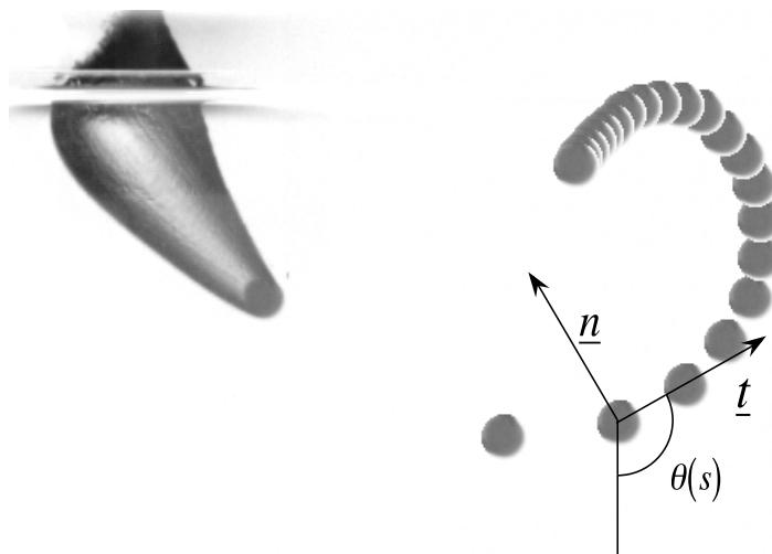
Figure 1. Chronophotography of the impact of an iso-density sphere ( R = 3.5 mm) penetrating a bath of water at U_0 = 35 m s ^{-1} and spinning at \omega_0 \approx 1200 rad s ^{-1} . The time step between images is not constant. t = 0 is the impact time, t_1 = -0.5 ms, t_2 = 2.8 ms, t_3 = 13 ms, t_4 = 42 ms, t_5 = 76 ms, t_6 = 101 ms, t_7 = 169 ms and t_8 = 216 ms. The arrows indicate the sphere velocity.
